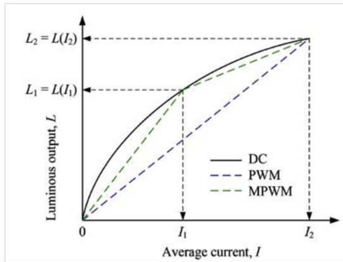
Figure 2: Light output characteristics under three driving methods
