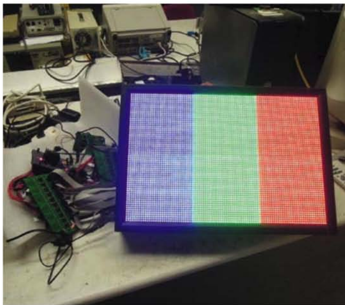
Figure 5: Prototype of an LED display panel with 2 \times 3 display modules
