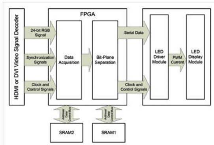
Figure 3: Conventional LED display panel system architecture
