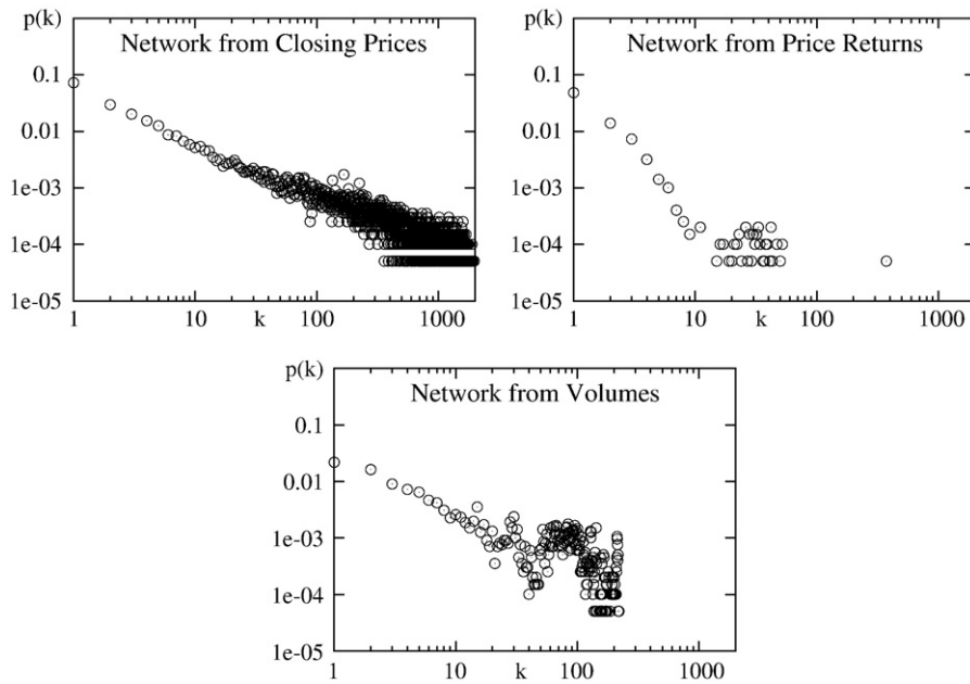
Fig. 2. Scalefree degree distribution of networks formed by a winner-take-all connection criterion with \rho=0.9 applied to cross correlation of daily closing prices (upper left panel); daily price returns (upper right panel); and daily trading volumes (lower panel), using Set 1 data.
